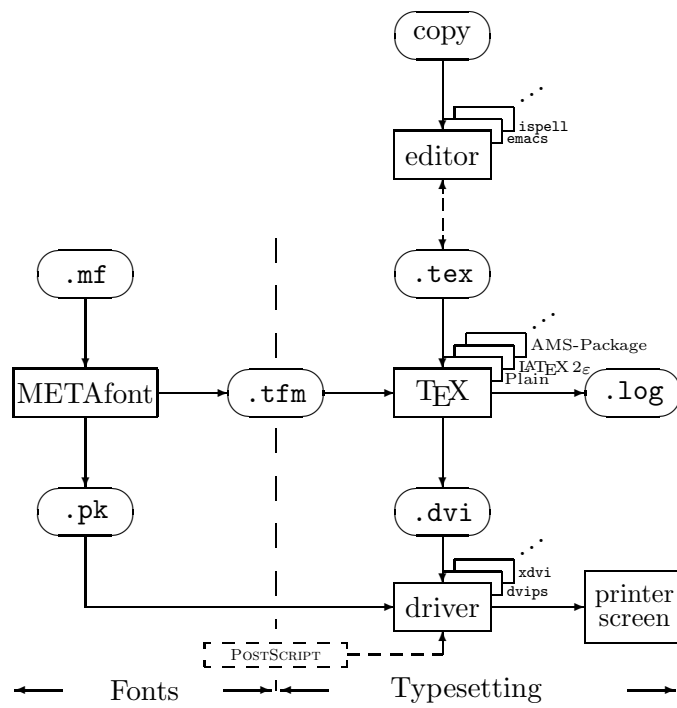
Figure 1.1: Components of a TeX system
