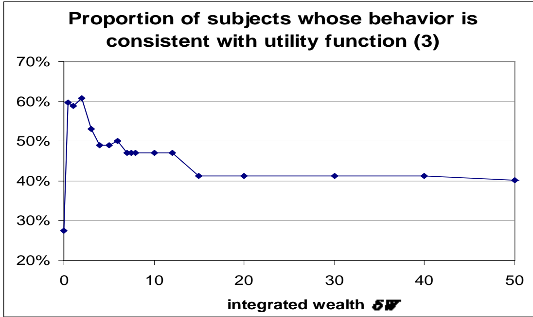
Figure 3. Proportion of subjects whose behavior is consistent with utility function (3). Non-robust cases counted as inconsistent. Data from Harrison et al. (2005).
