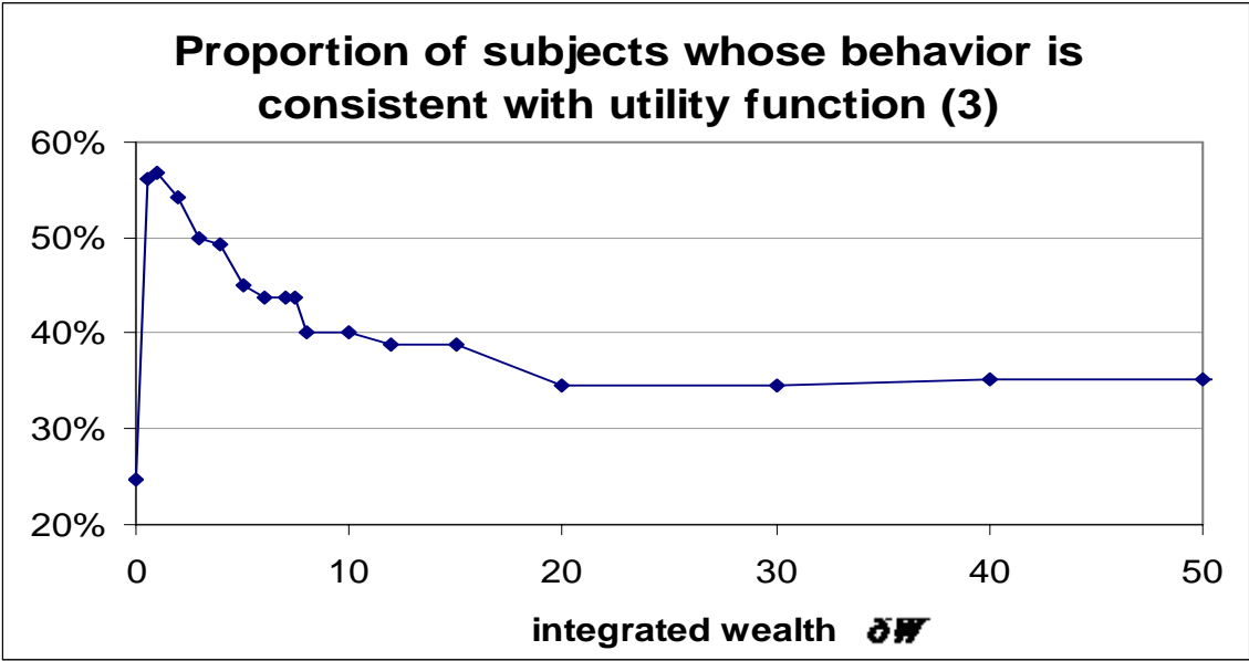
Figure 2. Proportion of subjects whose behavior is consistent with utility function (3). Non-robust cases counted as inconsistent. Data from Holt and Laury (2002b).
