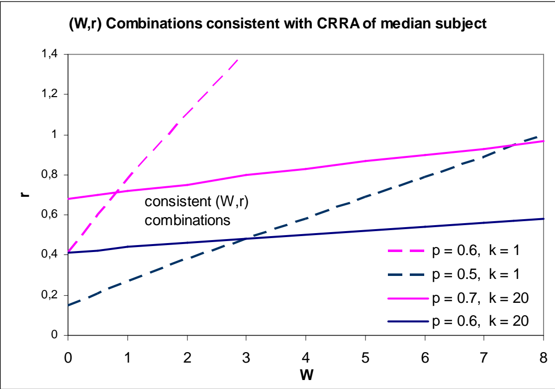
Figure 1. (W, r) combinations that are consistent with CRRA of subject with median number of safe choices in both treatments.
